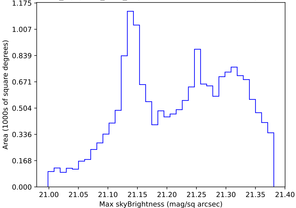
noroll_mjdp180_v3.4_10yrs WFD r band: Max skyBrightness
