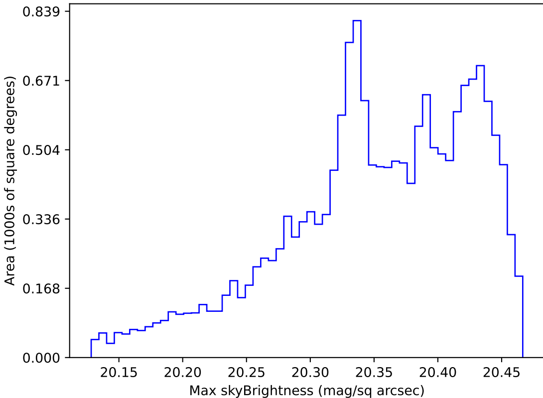
noroll_mjdp180_v3.4_10yrs WFD i band: Max skyBrightness
