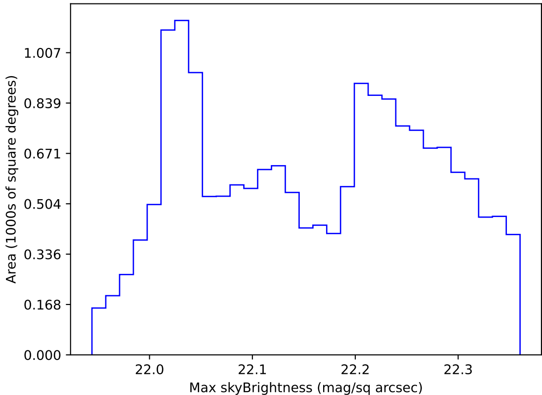
noroll_mjdp180_v3.4_10yrs WFD g band: Max skyBrightness
