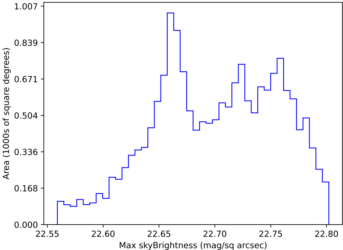
noroll_mjdp180_v3.4_10yrs WFD all bands: Max skyBrightness
