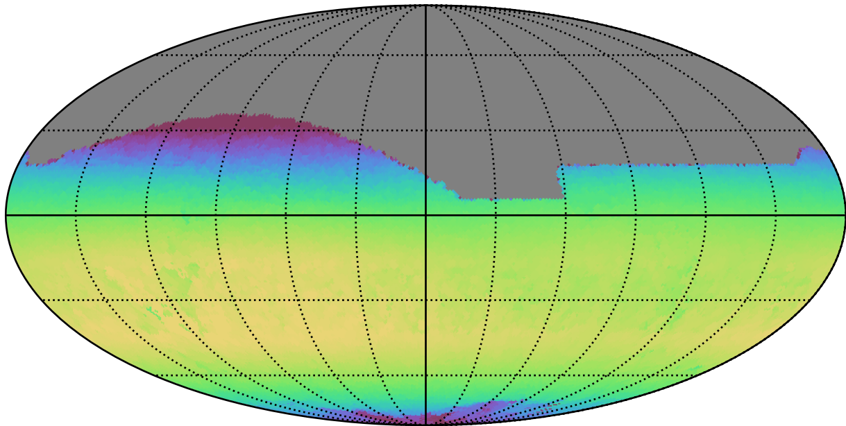
noroll_mjdp180_v3.4_10yrs All sky z band: Max skyBrightness
