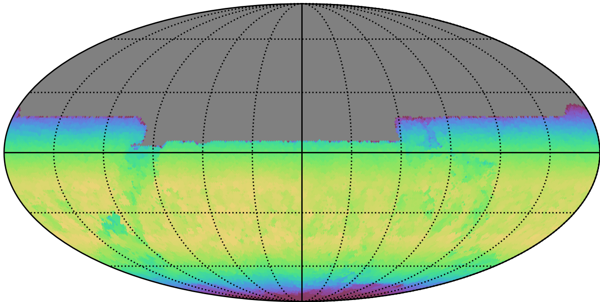
noroll_mjdp180_v3.4_10yrs All sky y band: Max skyBrightness
