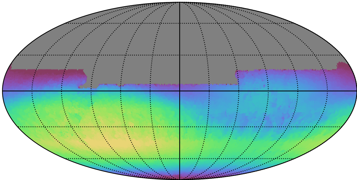
noroll_mjdp180_v3.4_10yrs All sky u band: Max skyBrightness
