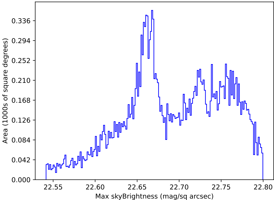
noroll_mjdp180_v3.4_10yrs All sky u band: Max skyBrightness
