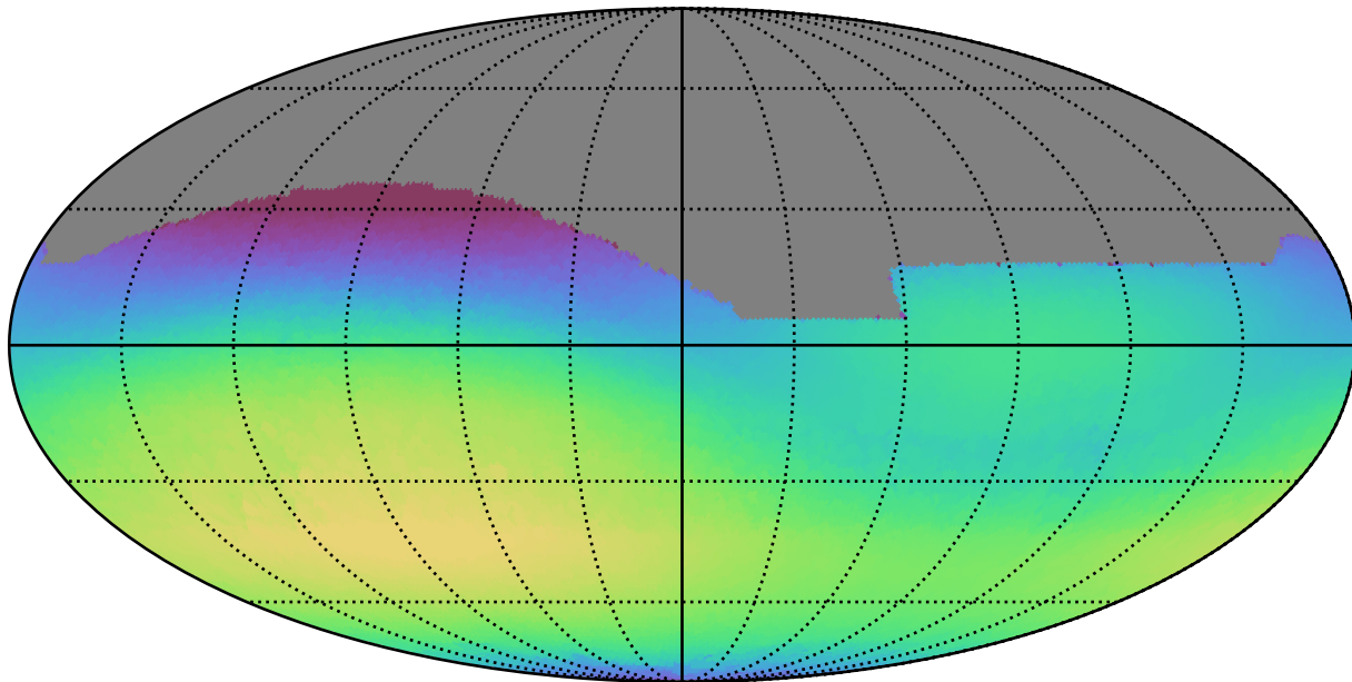
noroll_mjdp180_v3.4_10yrs All sky r band: Max skyBrightness
