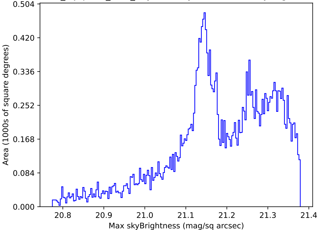
noroll_mjdp180_v3.4_10yrs All sky r band: Max skyBrightness
