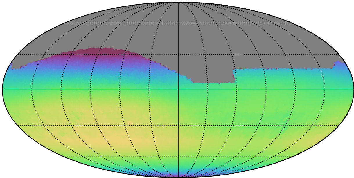
noroll_mjdp180_v3.4_10yrs All sky i band: Max skyBrightness
