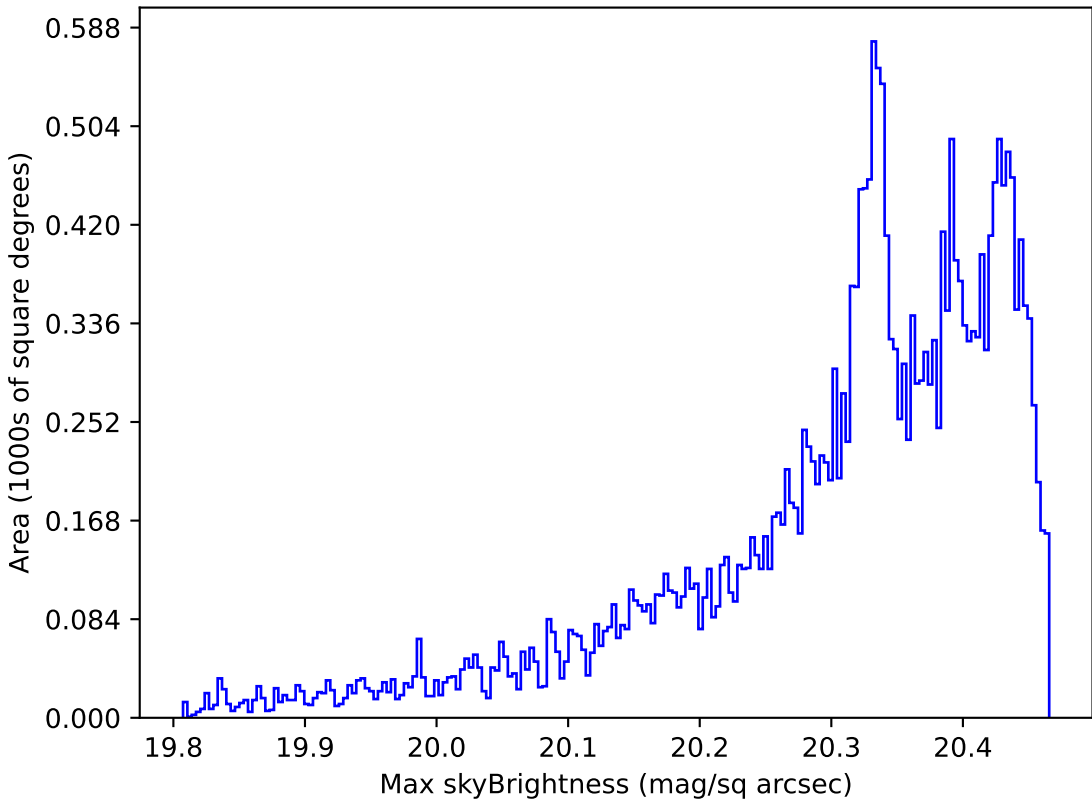
noroll_mjdp180_v3.4_10yrs All sky i band: Max skyBrightness
