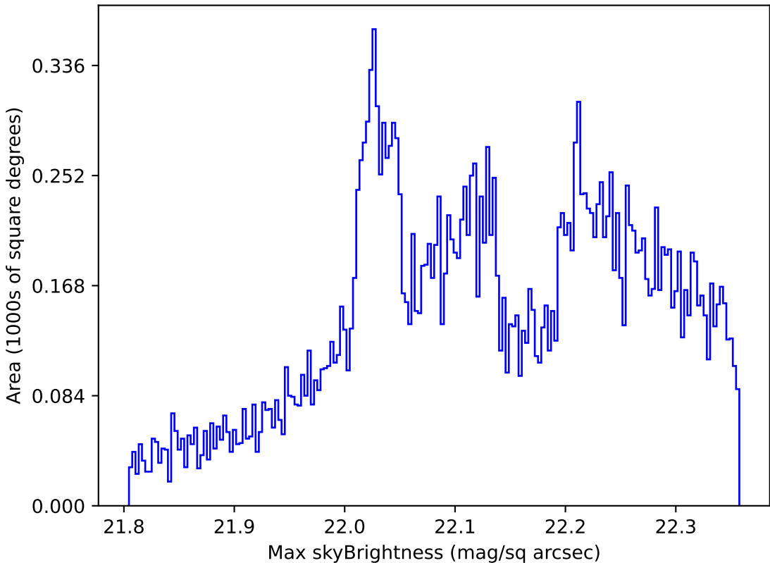
noroll_mjdp180_v3.4_10yrs All sky g band: Max skyBrightness
