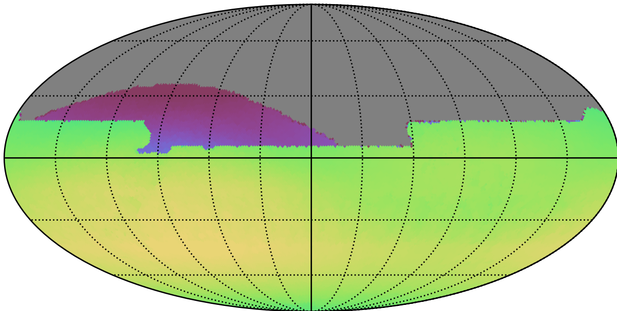
noroll_mjdp180_v3.4_10yrs All sky all bands: Max skyBrightness
