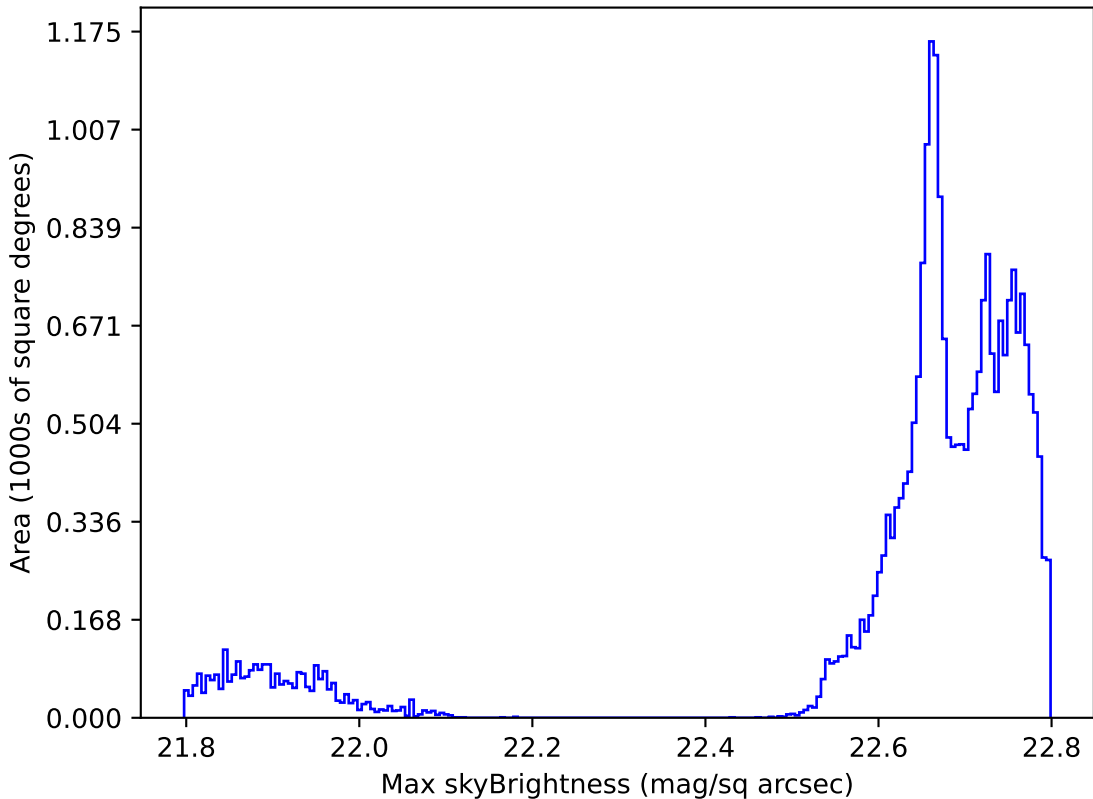
noroll_mjdp180_v3.4_10yrs All sky all bands: Max skyBrightness
