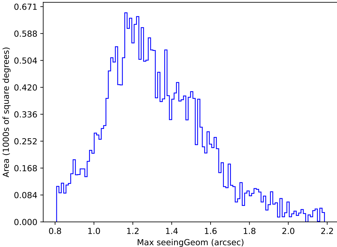
noroll_mjdp180_v3.4_10yrs Yr 1 z band: Max seeingGeom
