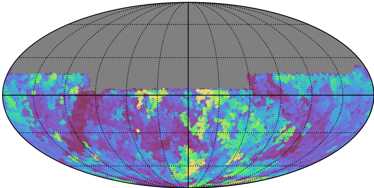
noroll_mjdp180_v3.4_10yrs Yr 1 y band: Max seeingGeom
