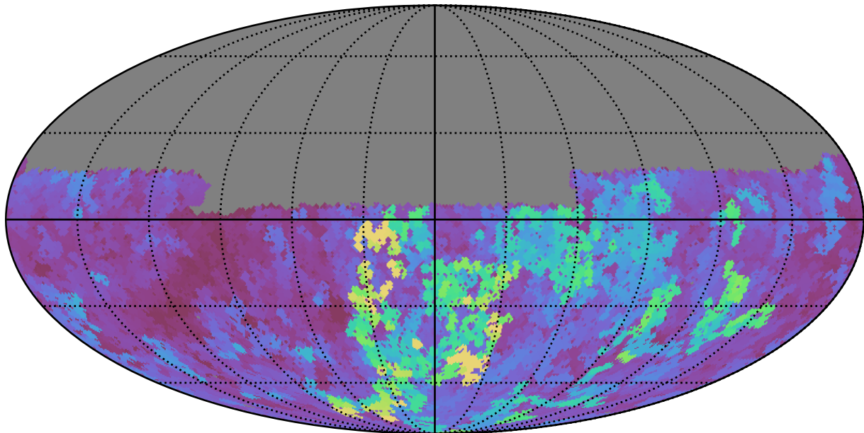
noroll_mjdp180_v3.4_10yrs Yr 1 u band: Max seeingGeom
