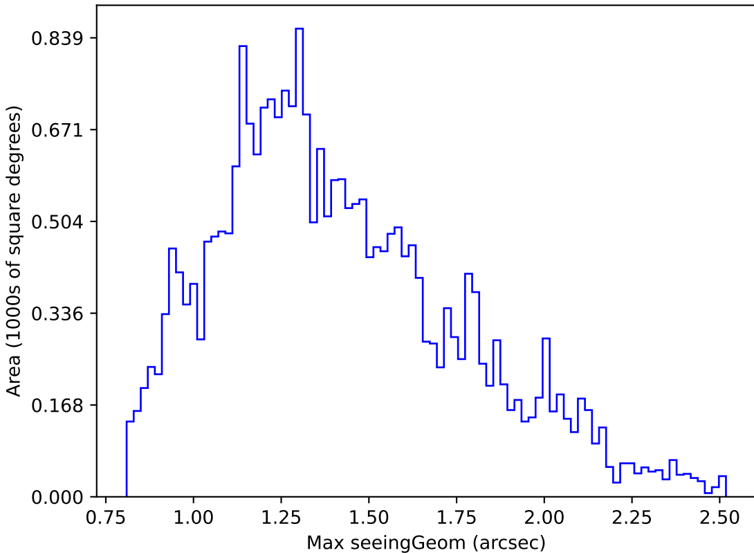
noroll_mjdp180_v3.4_10yrs Yr 1 r band: Max seeingGeom
