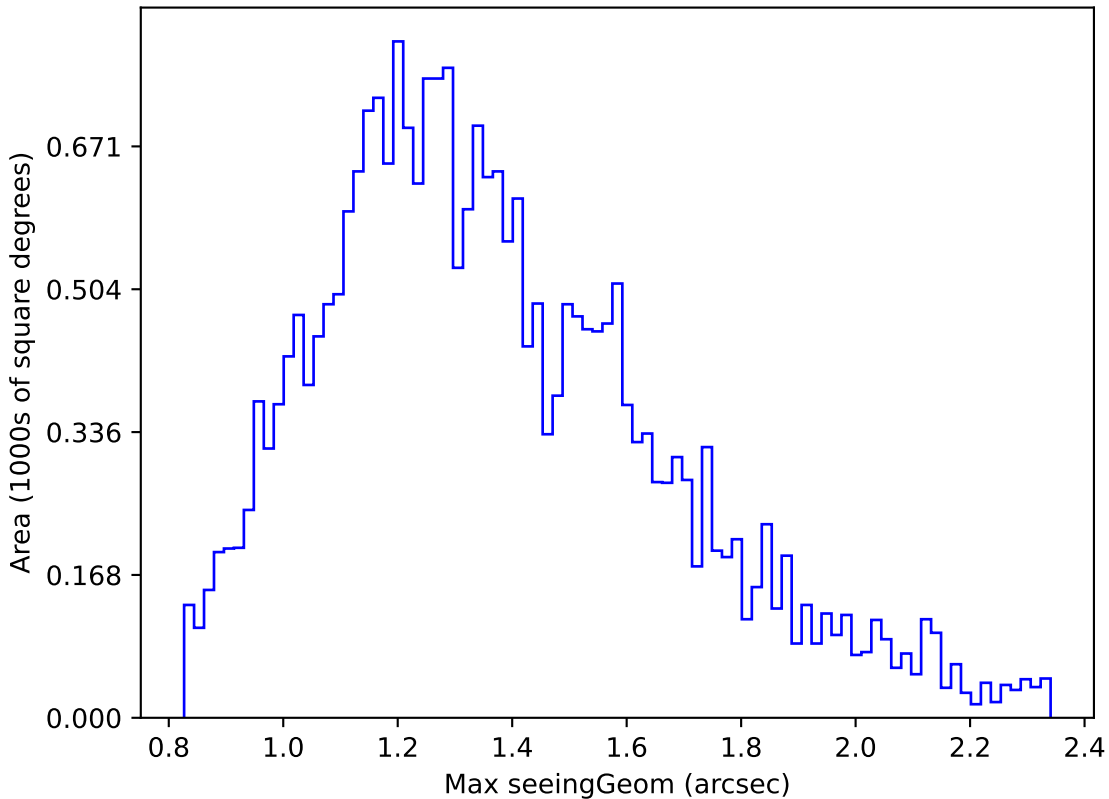
noroll_mjdp180_v3.4_10yrs Yr 1 i band: Max seeingGeom
