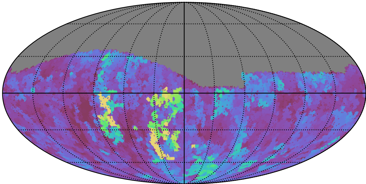
noroll_mjdp180_v3.4_10yrs Yr 1 g band: Max seeingGeom
