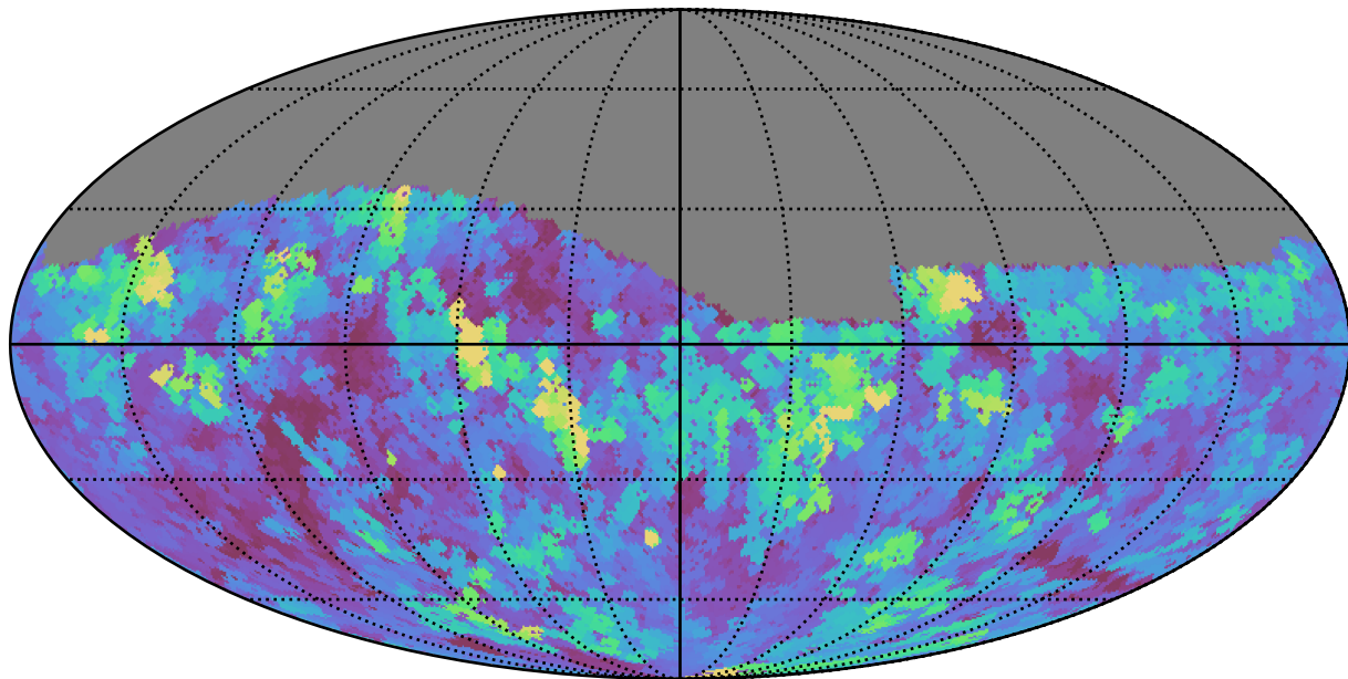
noroll_mjdp180_v3.4_10yrs Yr 1 z band: Max seeingEff
