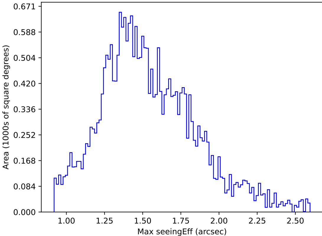
noroll_mjdp180_v3.4_10yrs Yr 1 z band: Max seeingEff
