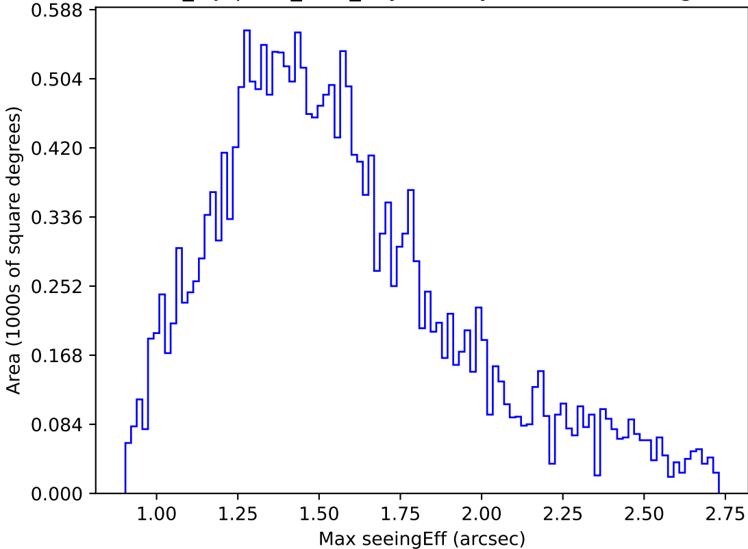
noroll_mjdp180_v3.4_10yrs Yr 1 y band: Max seeingEff
