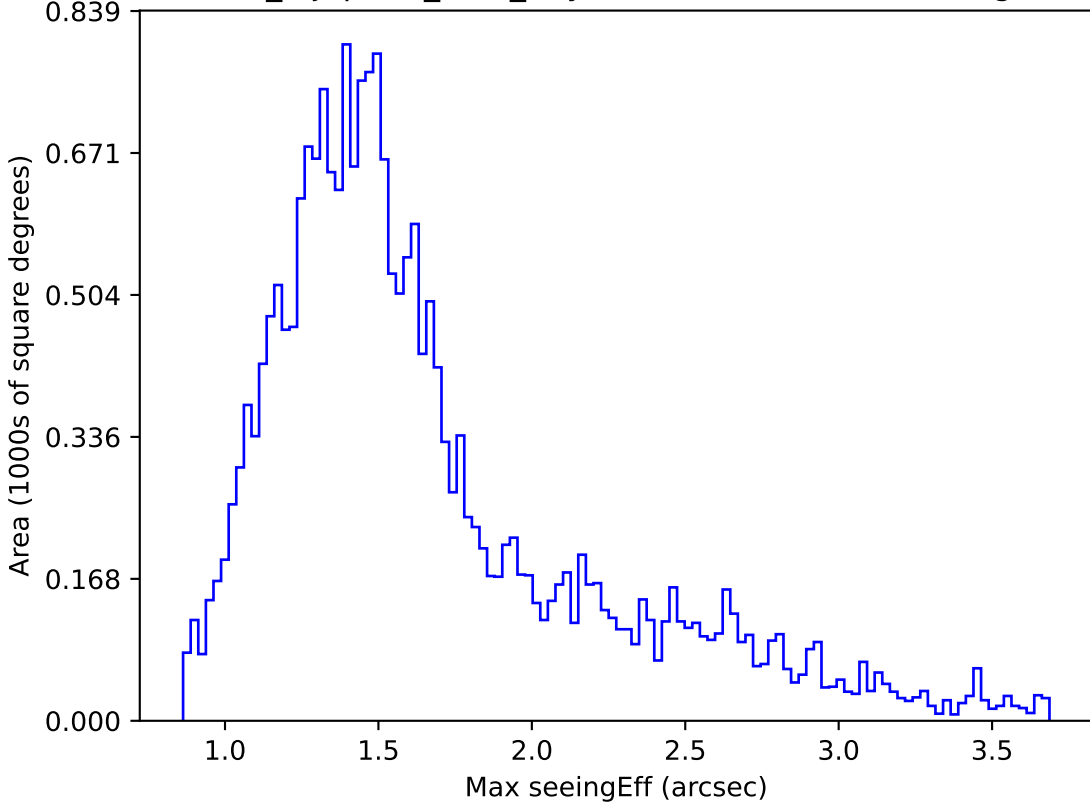
noroll_mjdp180_v3.4_10yrs Yr 1 u band: Max seeingEff
