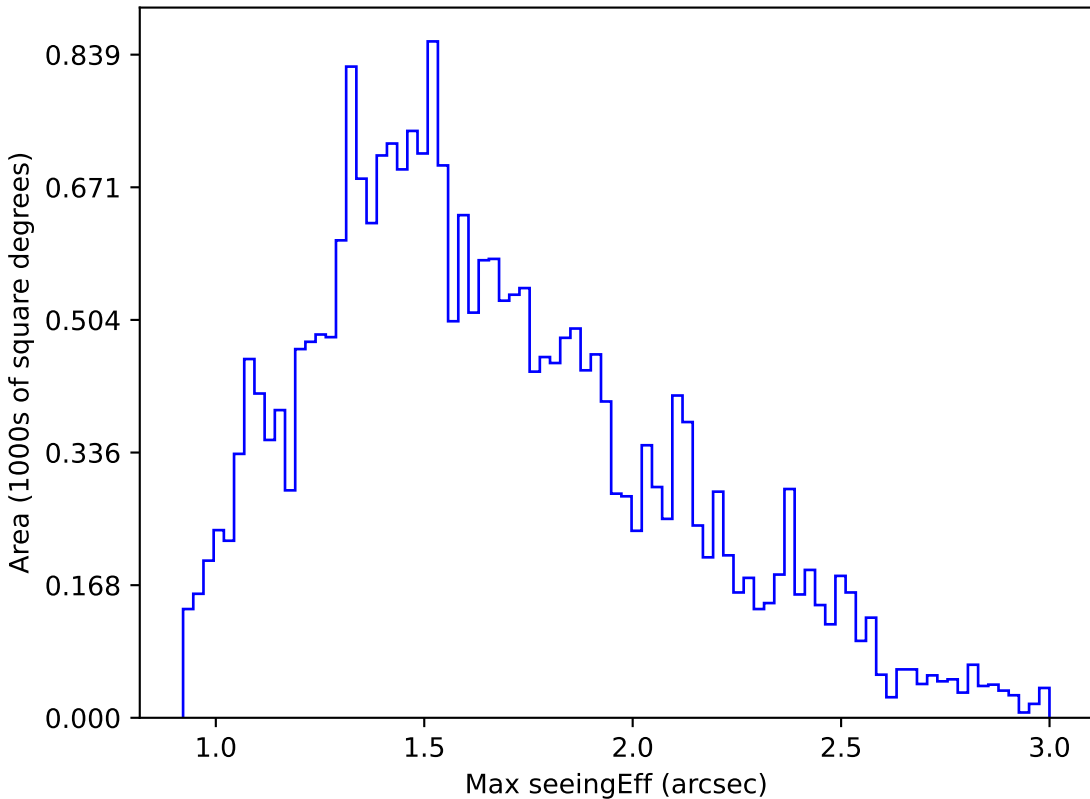
noroll_mjdp180_v3.4_10yrs Yr 1 r band: Max seeingEff
