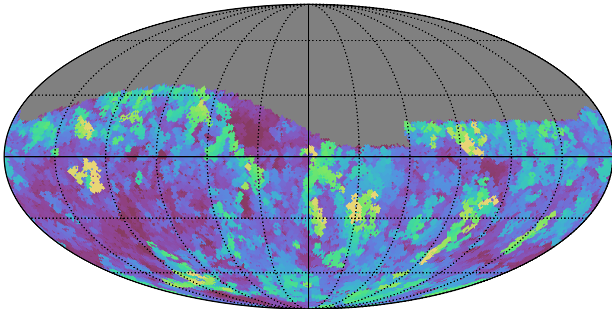
noroll_mjdp180_v3.4_10yrs Yr 1 i band: Max seeingEff
