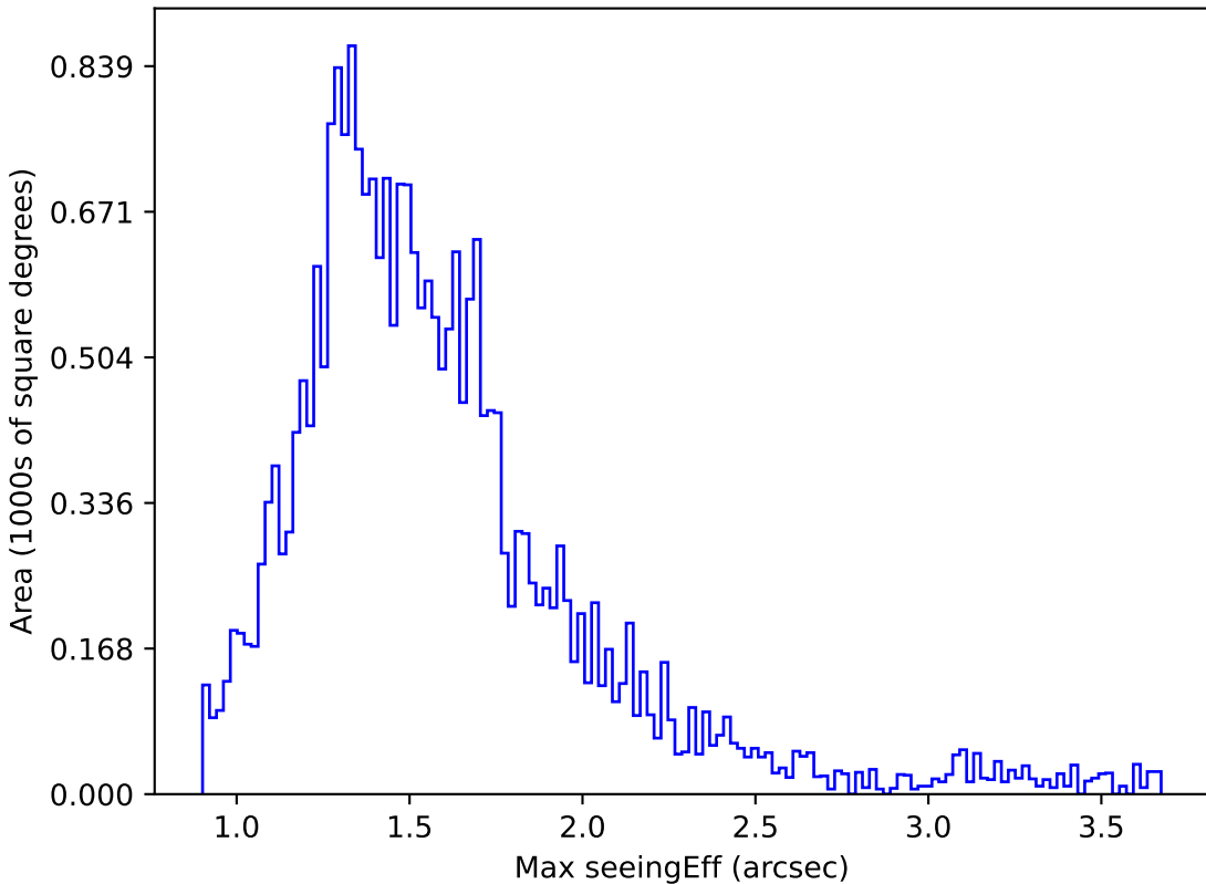
noroll_mjdp180_v3.4_10yrs Yr 1 g band: Max seeingEff
