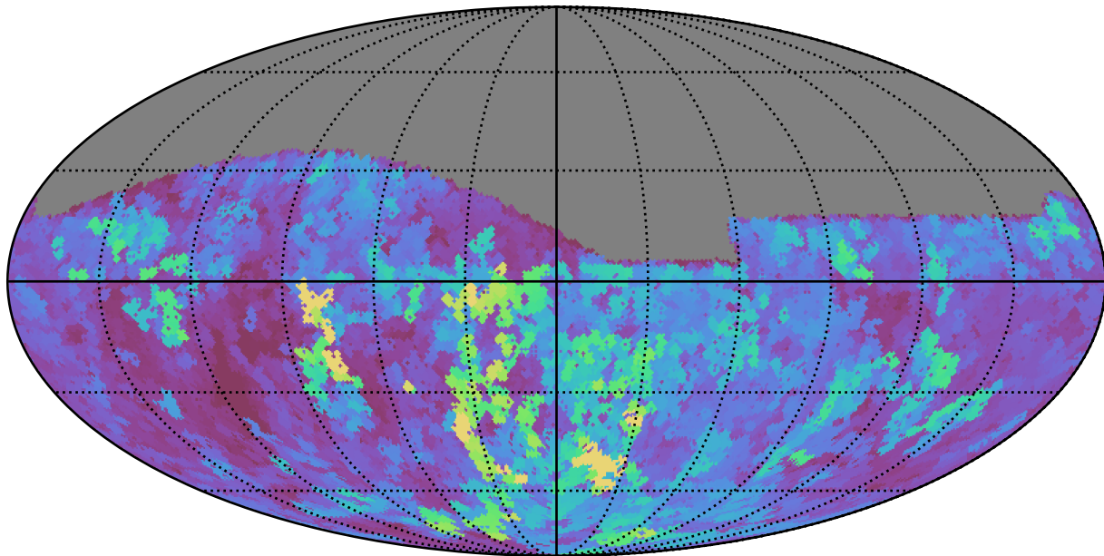
noroll_mjdp180_v3.4_10yrs Yr 1 all bands: Max seeingEff
