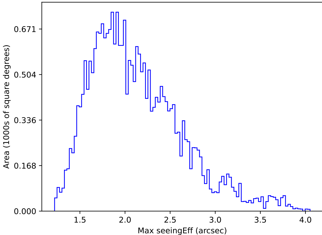
noroll_mjdp180_v3.4_10yrs Yr 1 all bands: Max seeingEff
