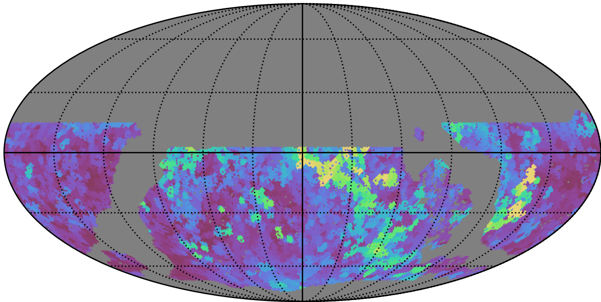
noroll_mjdp180_v3.4_10yrs WFD y band: Max seeingEff
