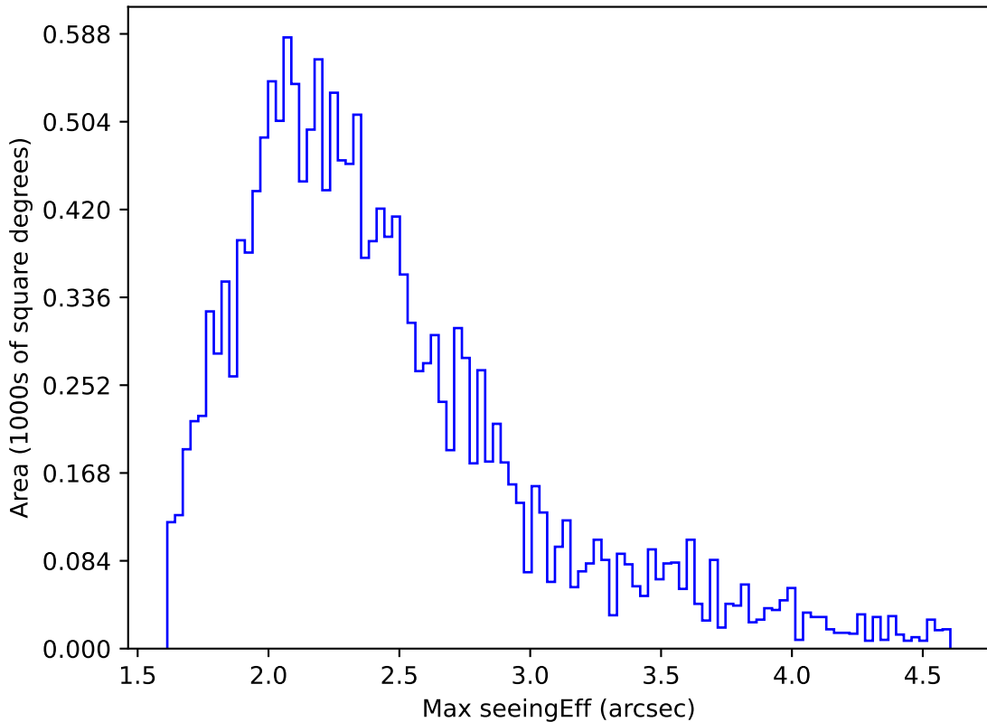
noroll_mjdp180_v3.4_10yrs WFD y band: Max seeingEff
