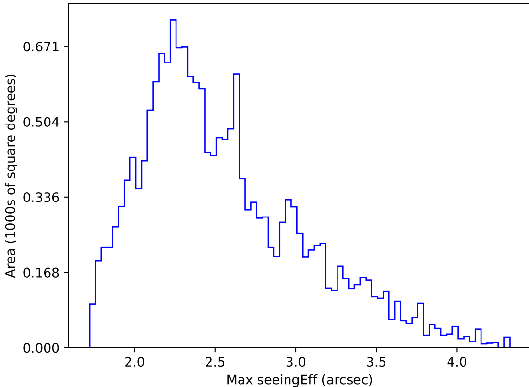
noroll_mjdp180_v3.4_10yrs WFD u band: Max seeingEff
