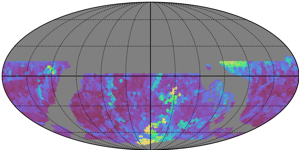
noroll_mjdp180_v3.4_10yrs WFD r band: Max seeingEff
