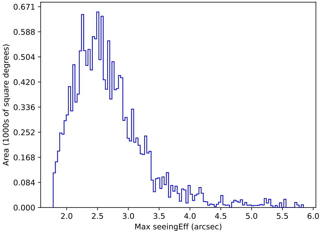
noroll_mjdp180_v3.4_10yrs WFD r band: Max seeingEff
