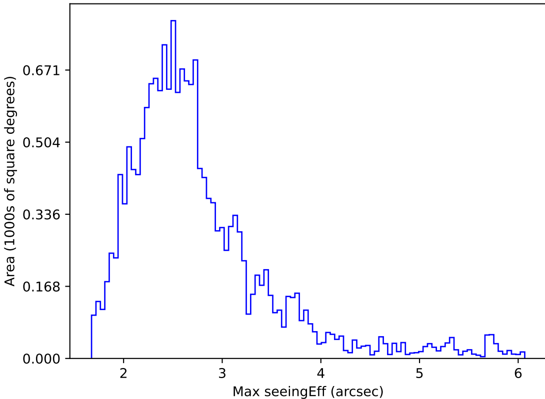
noroll_mjdp180_v3.4_10yrs WFD i band: Max seeingEff
