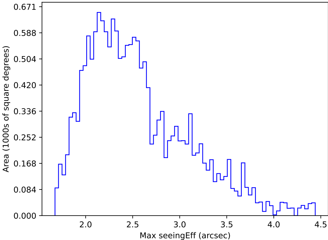
noroll_mjdp180_v3.4_10yrs WFD g band: Max seeingEff
