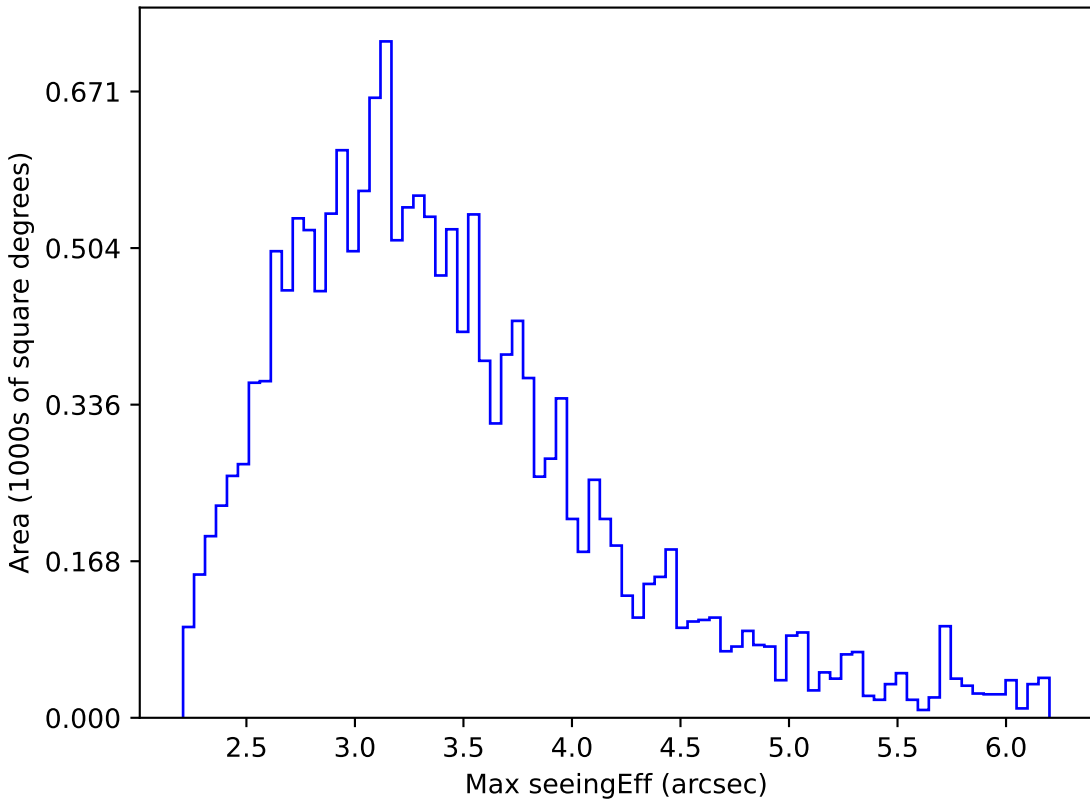
noroll_mjdp180_v3.4_10yrs WFD all bands: Max seeingEff
