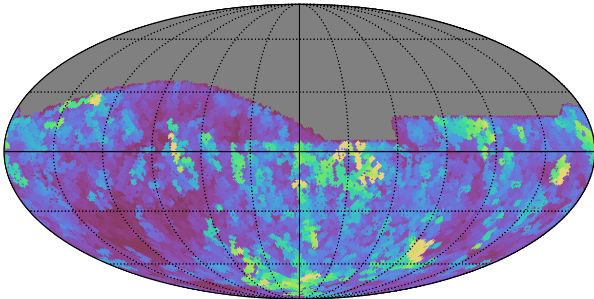
noroll_mjdp180_v3.4_10yrs All sky z band: Max seeingEff
