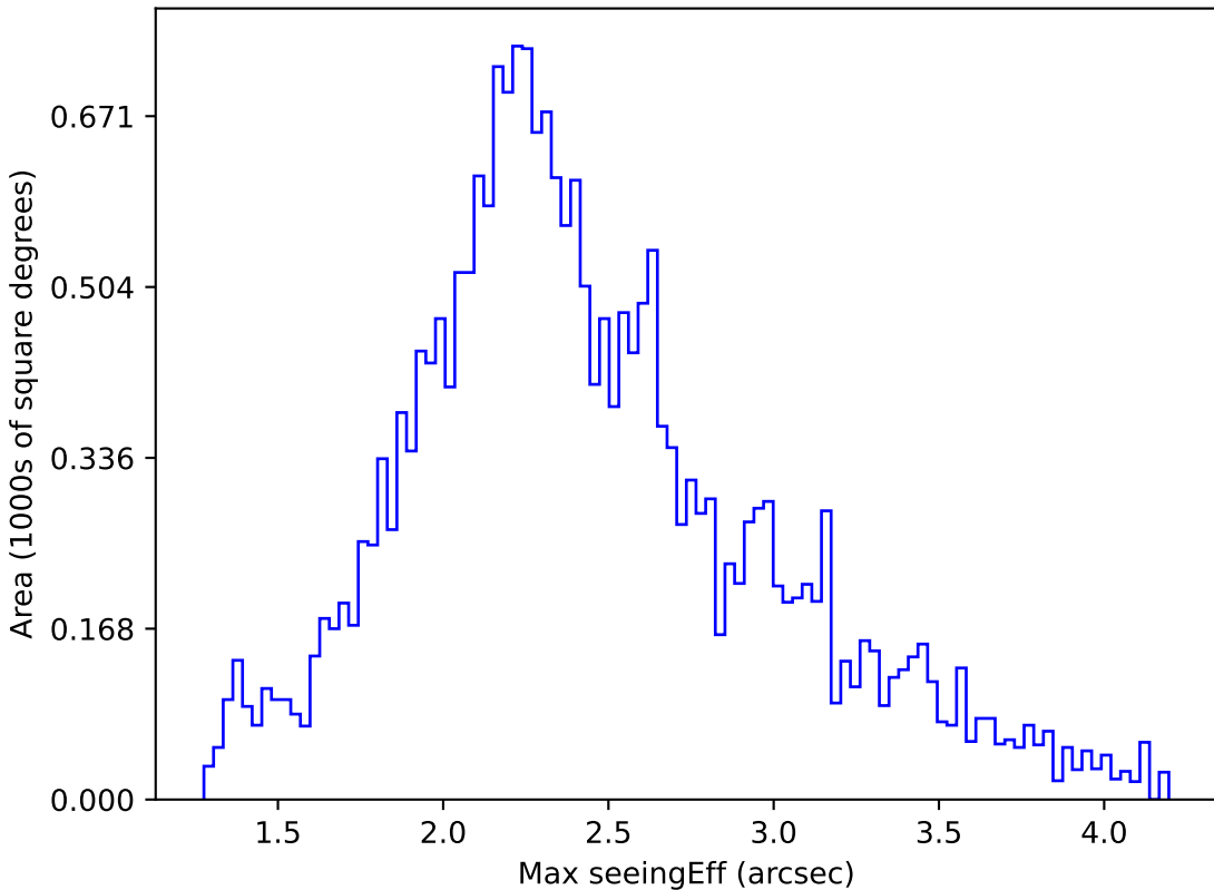
noroll_mjdp180_v3.4_10yrs All sky u band: Max seeingEff
