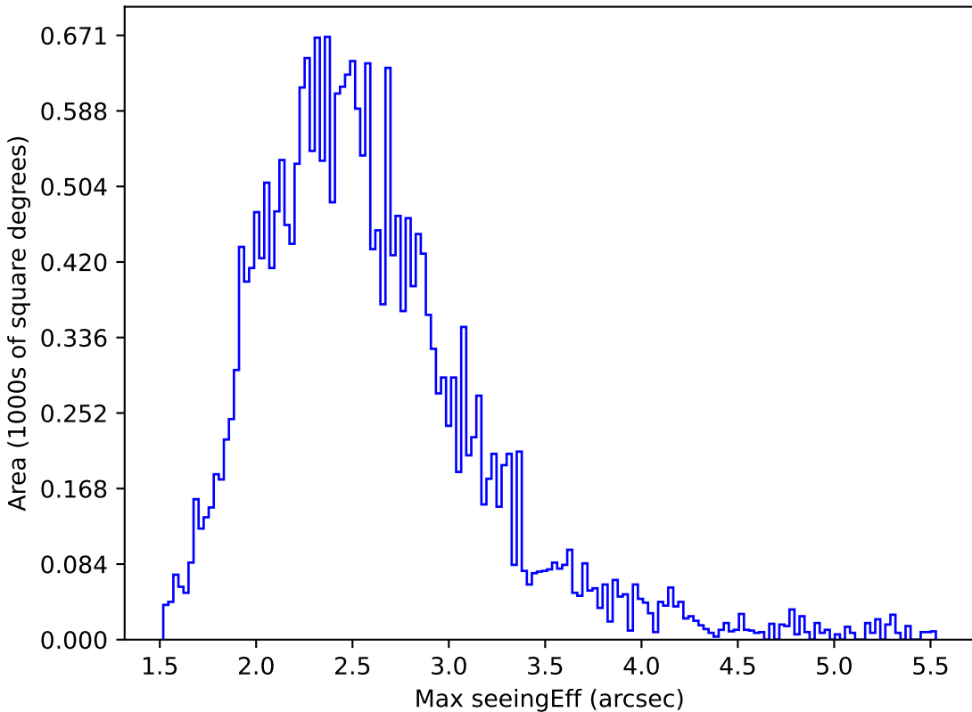
noroll_mjdp180_v3.4_10yrs All sky r band: Max seeingEff
