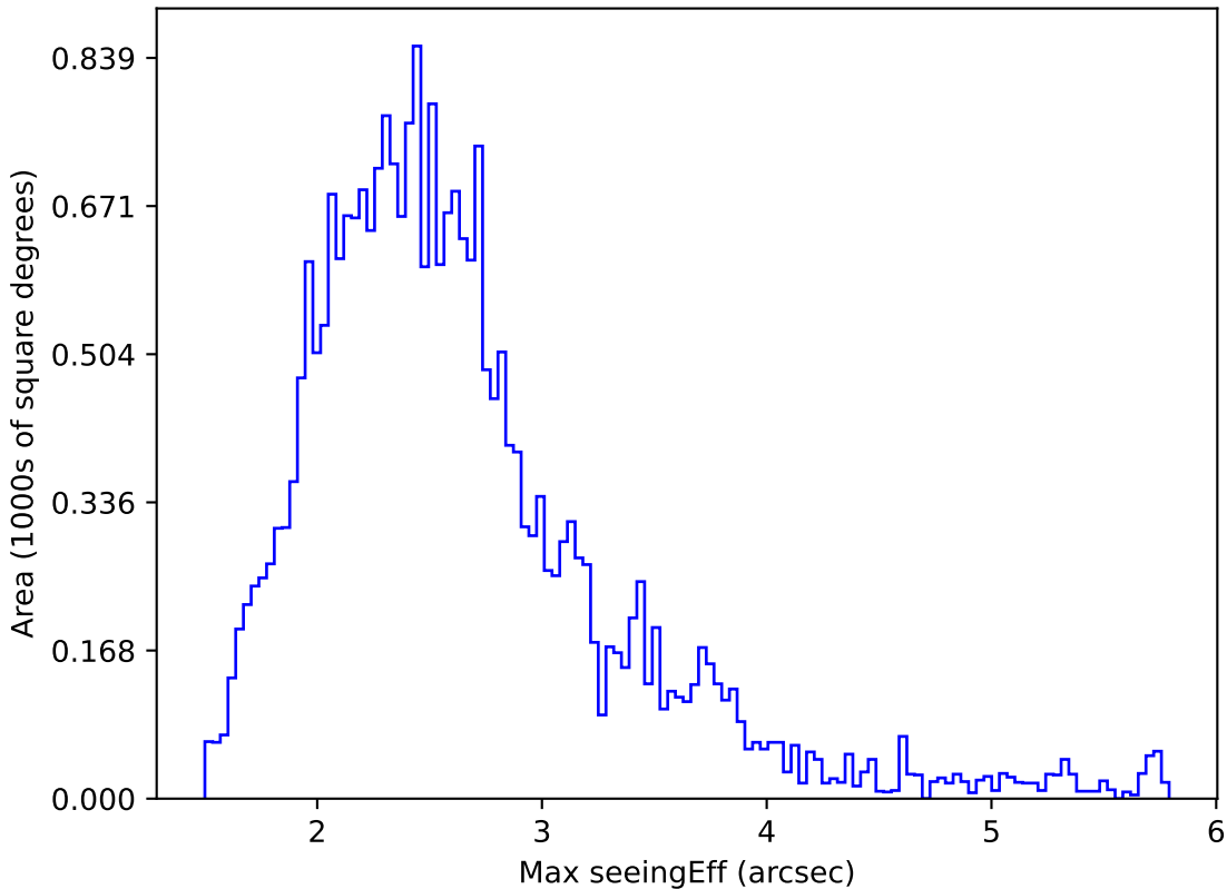
noroll_mjdp180_v3.4_10yrs All sky i band: Max seeingEff
