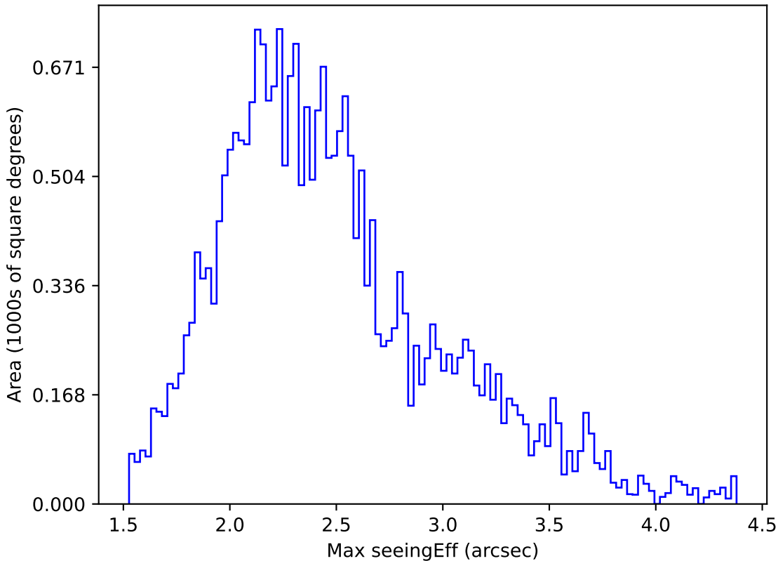
noroll_mjdp180_v3.4_10yrs All sky g band: Max seeingEff
