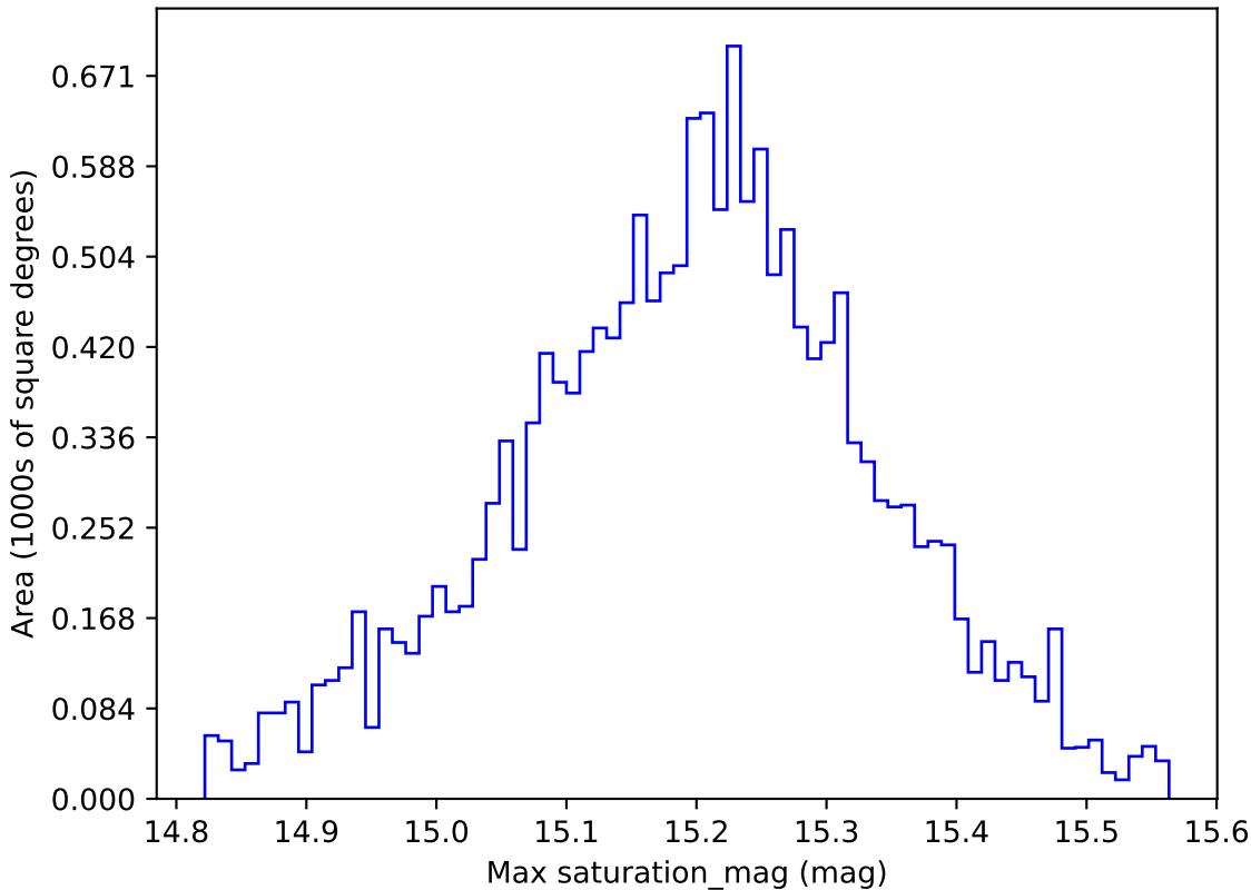
noroll_mjdp180_v3.4_10yrs WFD z band: Max saturation_mag
