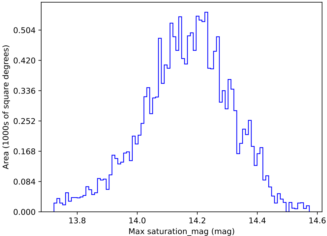
noroll_mjdp180_v3.4_10yrs WFD y band: Max saturation_mag
