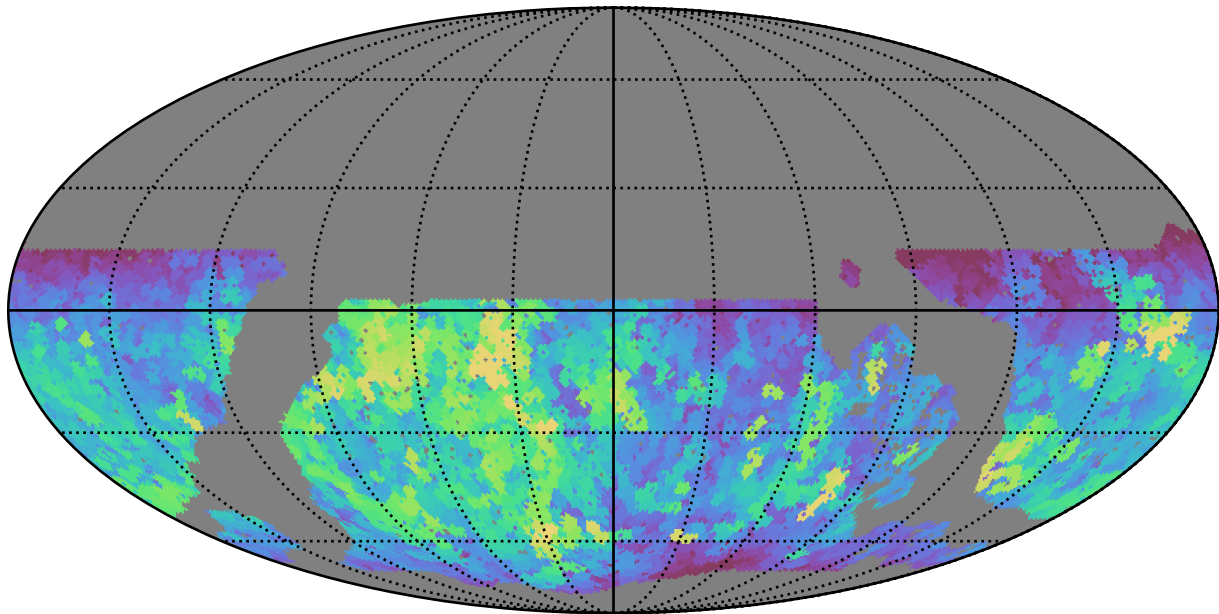
noroll_mjdp180_v3.4_10yrs WFD r band: Max saturation_mag
