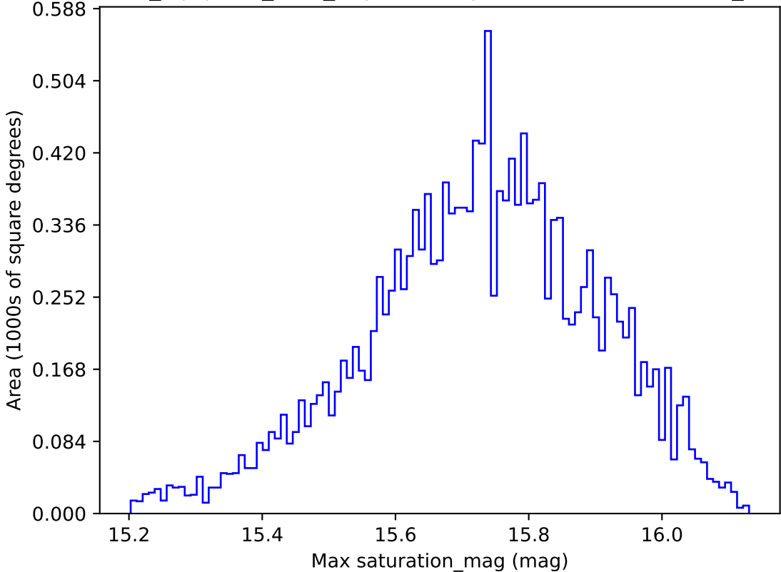
noroll_mjdp180_v3.4_10yrs WFD g band: Max saturation_mag
