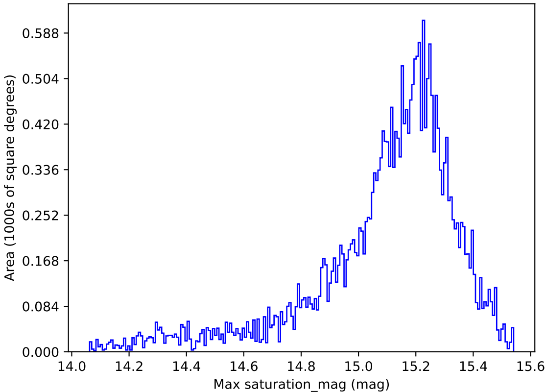
noroll_mjdp180_v3.4_10yrs All sky z band: Max saturation_mag
