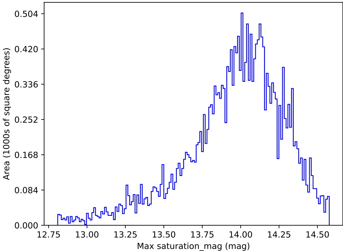
noroll_mjdp180_v3.4_10yrs All sky u band: Max saturation_mag
