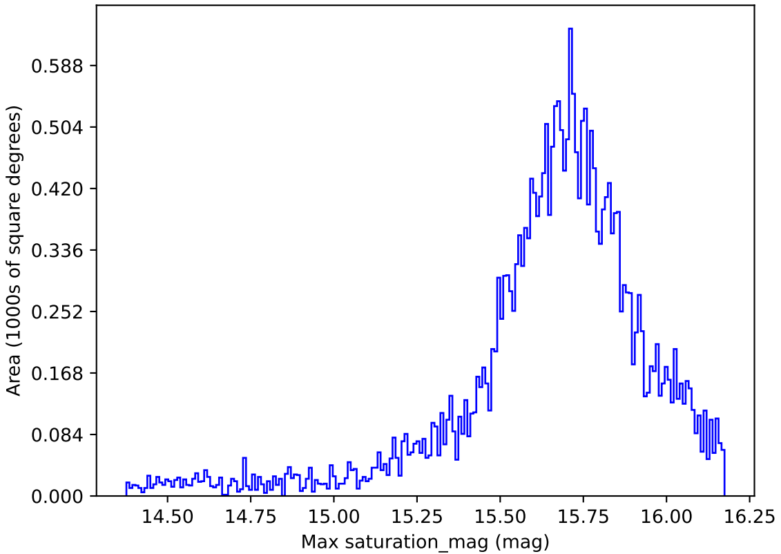
noroll_mjdp180_v3.4_10yrs All sky r band: Max saturation_mag
